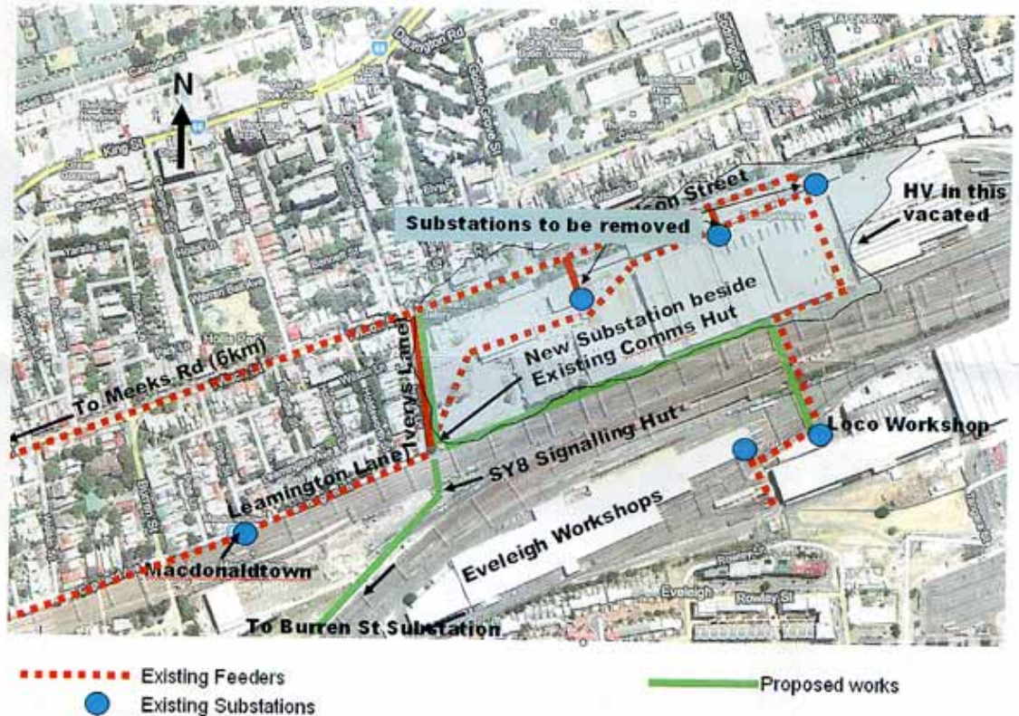
Figure 1: Location Plan/Layout Diagram
